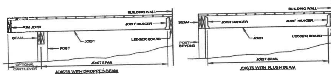
FIGURE AM106.1 TYPICAL DECK JOIST SPANS
